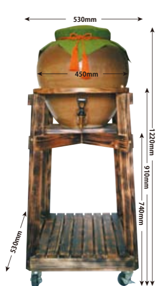
KK-36L + 専用SS木製台座
